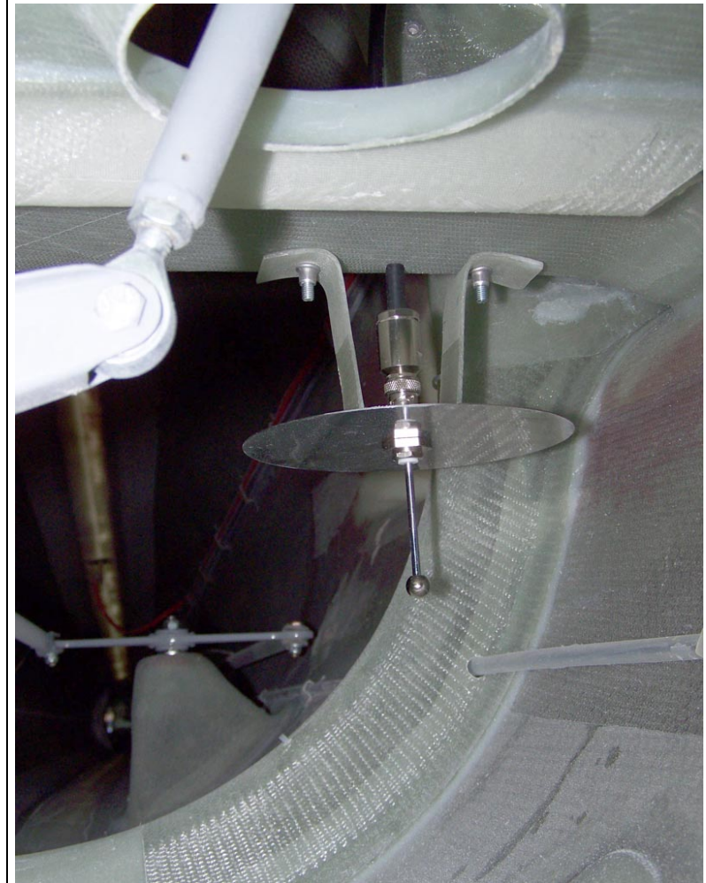
bracket, ground plate and antenna
