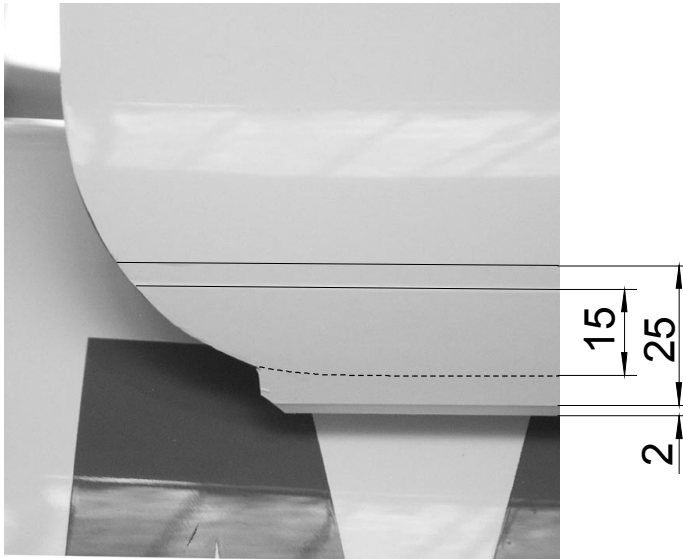
Fig. 10 Engine bay doors, rear end
