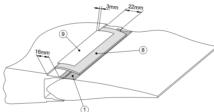
Fig. 2 (Horizontal tail upper surface)
